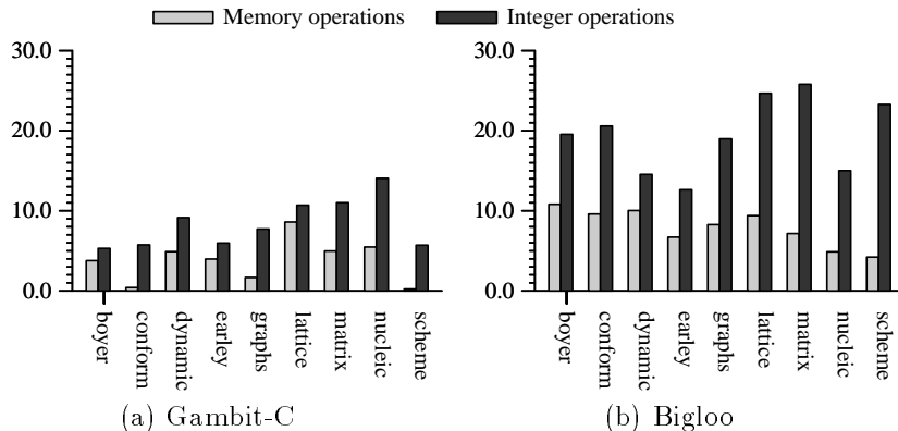
Fig. 4. Reduction in operations executed (%)
