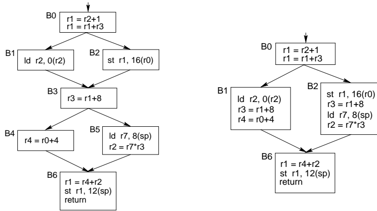
(b) Procedure obtained from the maximal matching (c) Procedure obtained after unmatching unprofitable instructions
