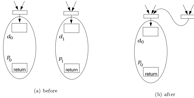
Fig. 4. Merging regions ending in return s via cross-jumping.
